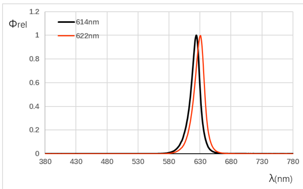
Fig 2. 相对发光光谱 / Relative Spectral Power Distribution vs. Wavelength
