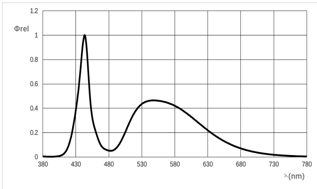
Fig 2. 相对发光光谱 Relative Spectral Distribution vs. Wavelength
